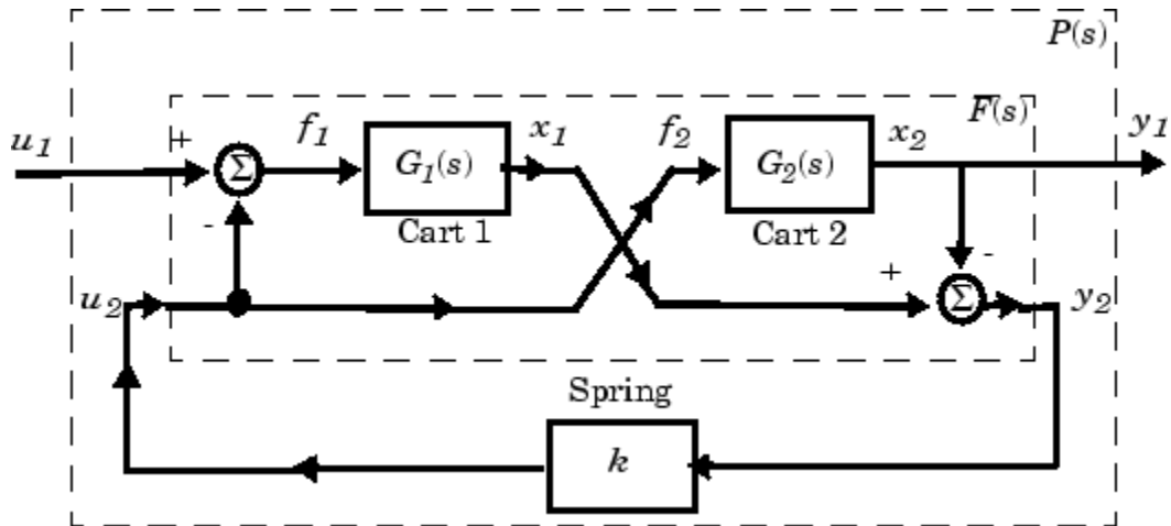
"ACC Benchmark" Two-Cart System Block Diagram y_1 = F(s) u_1
